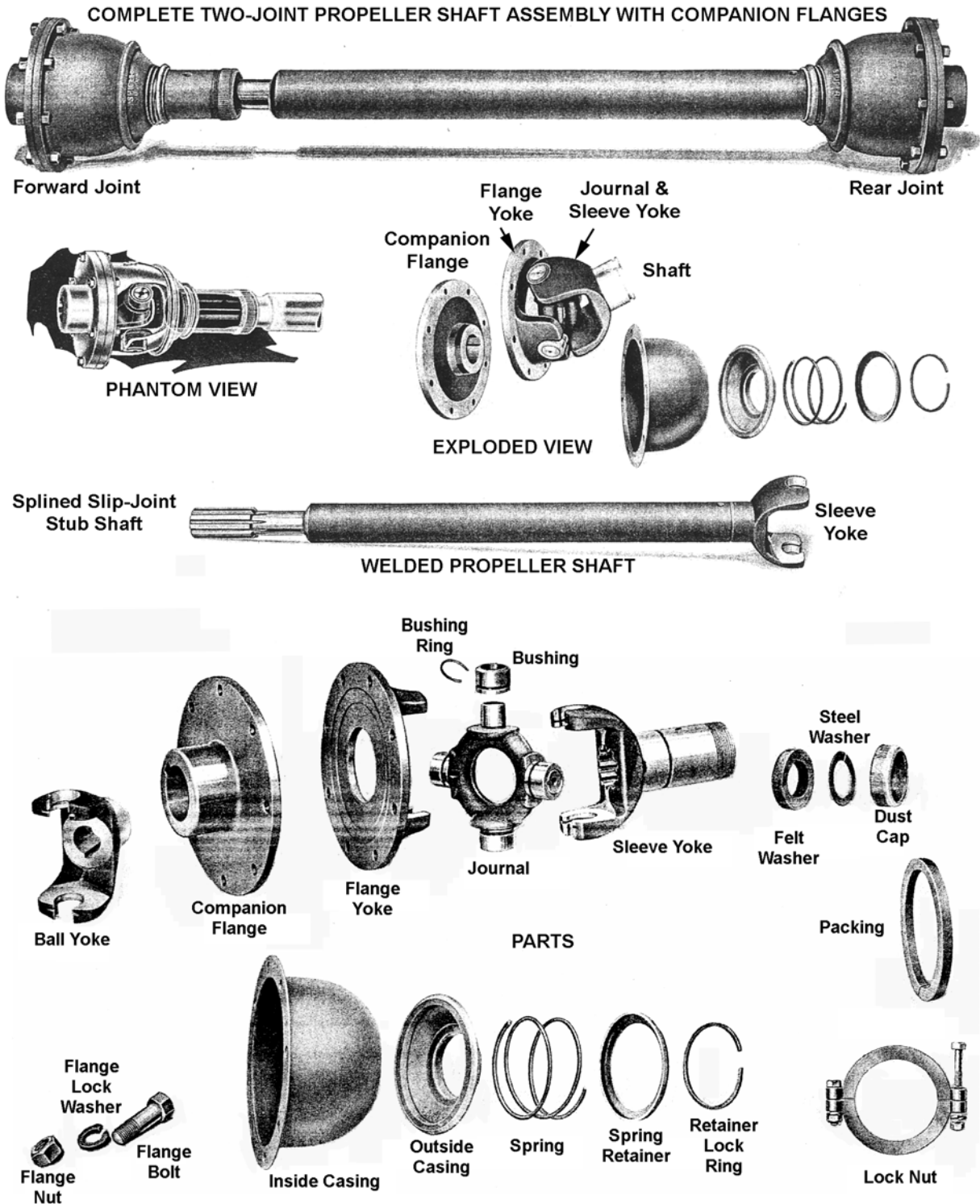
Figure 4. SPICER UNIVERSAL JOINT & PROPELLER SHAFT DETAILS
