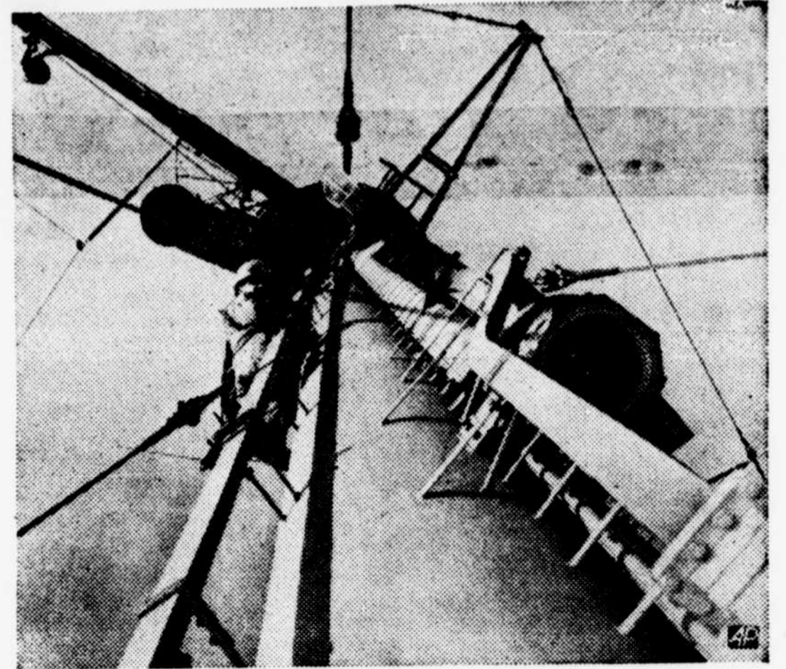
RADAR SPOUTS —Up the mainmast of the new cruiser USS Juneau, being built at a Kearny, N. J., shipyard, run these radar spouts which carry electric waves from the radar room of the vessel to broadcasting outlets above.
