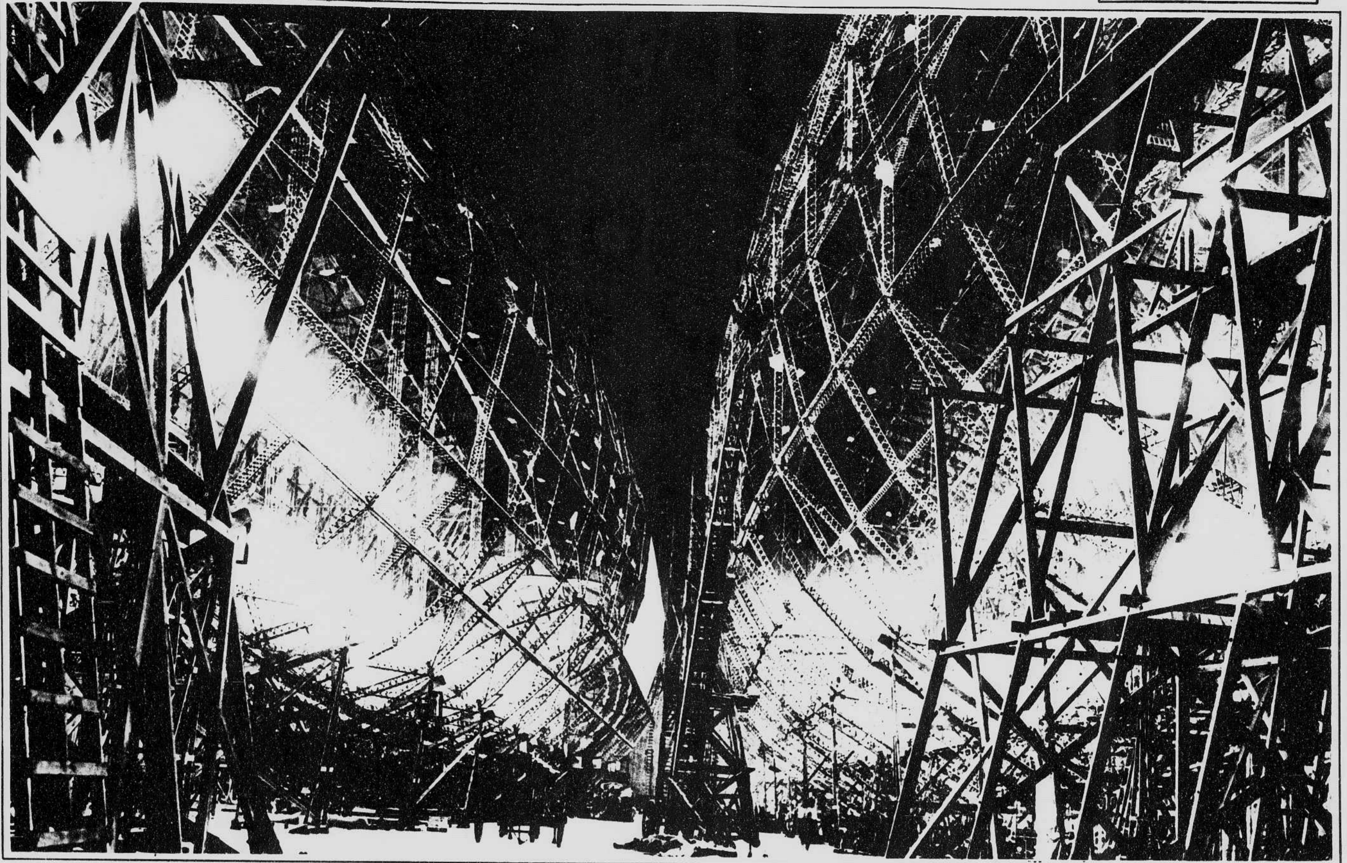
THE LARGEST AIRSHIP IN THE WORLD BUILDING FOR UNCLE SAM. At work on the giant dirigible R-38 (right), which is being built in England for the American navy. At present the 694-foot-long air monster is a fairy-like structure of delicate aluminum girders and latticework, but it is expected it will be in commission and ready to sail for America next spring. Her estimated maximum speed is 75 miles an hour. The largest hangar ever constructed is now building at Lakewood, N. J., to house the R-38. Central News
