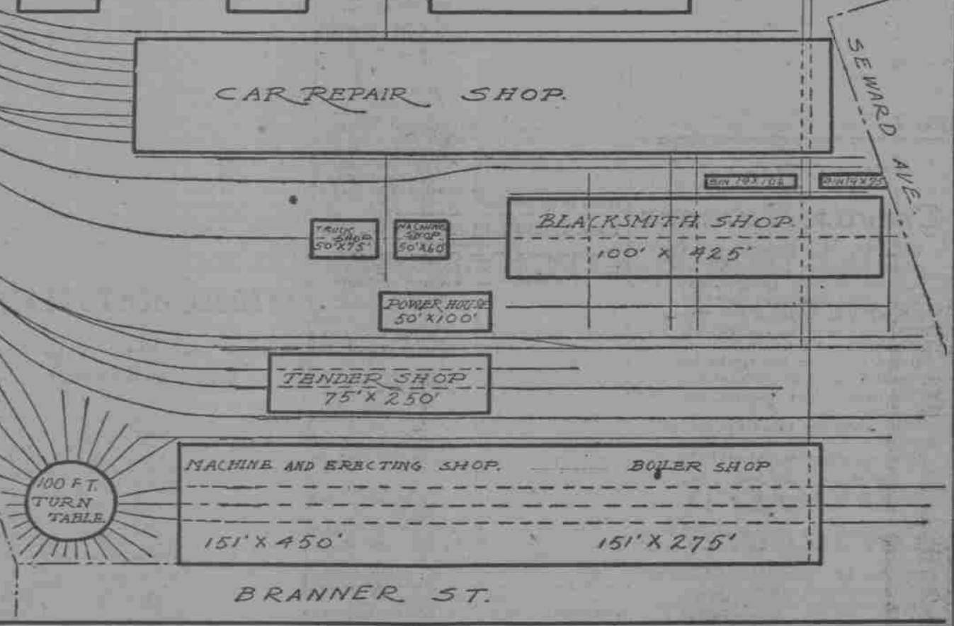
Revised Ground Plan of the Proposed Santa Fe Shop Extension.
