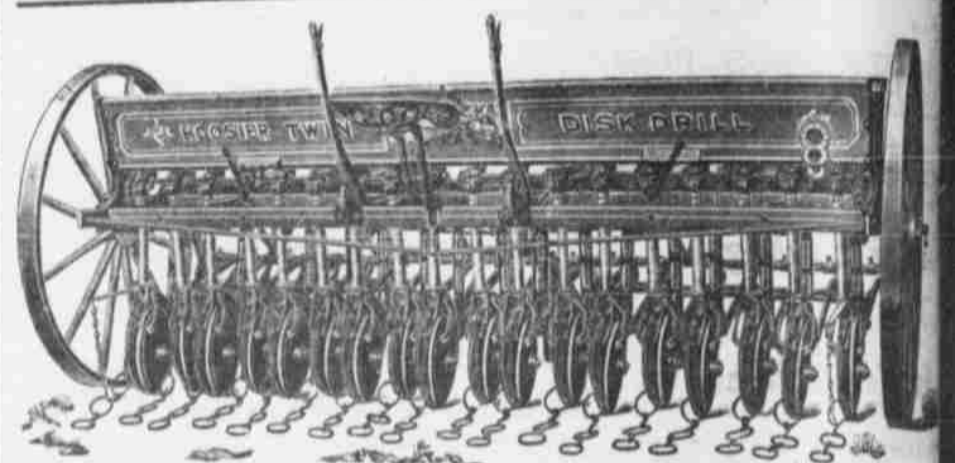
The Hoosier Positive Force Feed Drill.
