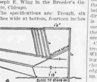
DIAGRAM OF RACK FOR FEEDING EWES WITH LAMBS.
